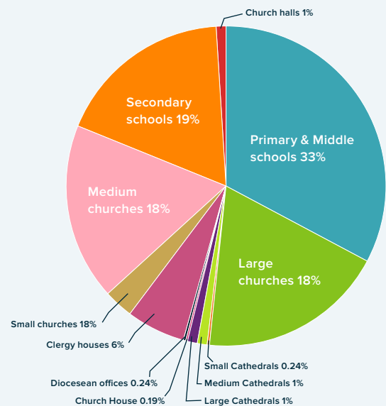
Breakdown of 2012 carbon footprint: % of total carbon emissions by building type
